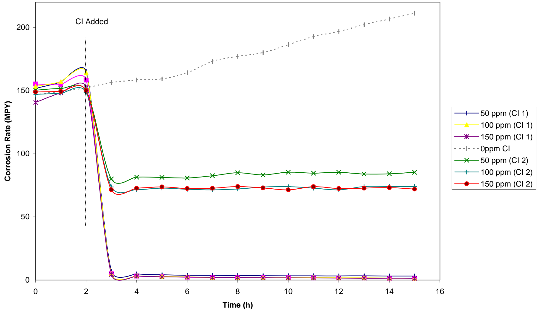
Comparison of the Corrosion Rate with Time for Cl's 1 & 2 at Various Concentrations Conditions: 50°C, CO 2 Sparged, in 3.5% NaCl Sea Water
